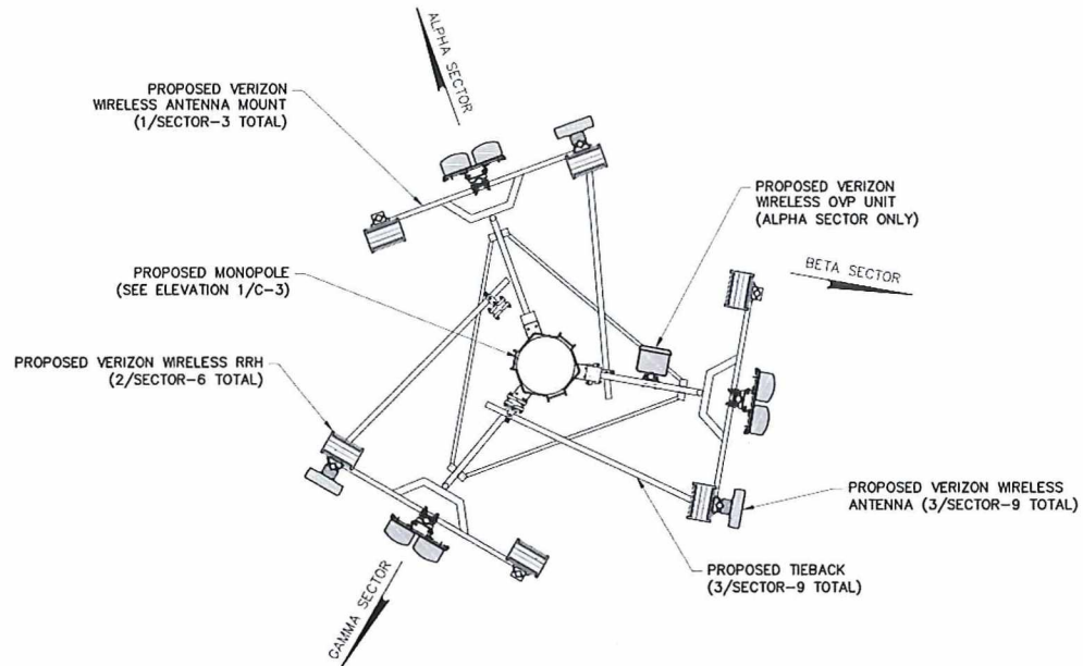
2 ANTENNA ORIENTATION SCALE: 3/16" = 1'-0" (11x17 SIZE) 3/8" = 1'-0" (22x34 SIZE)
